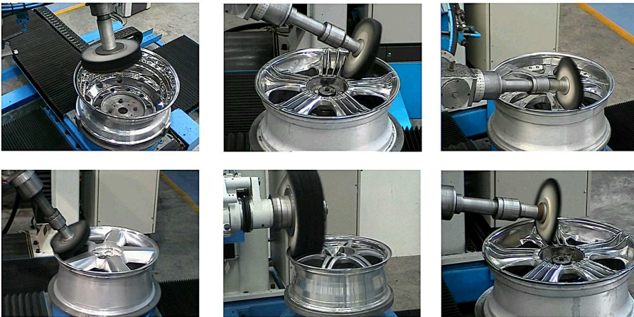
Examples of HD-II/2UT-CNC and rotary transfer machines polishing aluminium alloy wheels
